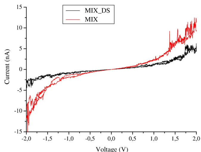
Fig. 5. I(V) curves of double-helical DNA 32-mers with mixed G, A, C, T sequences (Table 1, ds sample 3) and double-helical DNA 32-mers with mixed G, A, C, T sequences with three bases missing in the middle (MIX_DS, see Table 1, ds 4). Set point 0.1 nA, 0.1 V, measured in both voltage directions.
