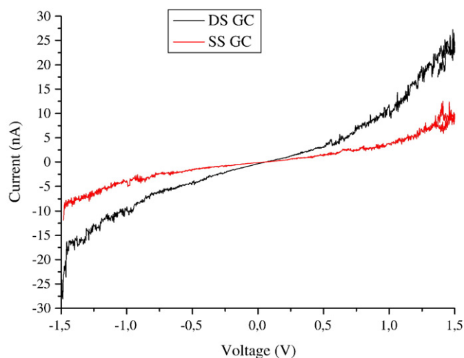
Fig. 4. The typical I(V) curves of DNA GC 32-base single strand (SS GC, see Table 1, SS A) and DNA GC 32-base double strand (DS GC, see Table 1, ds 1). Set point 0.1 nA, 0.1 V, measured in one voltage direction.
