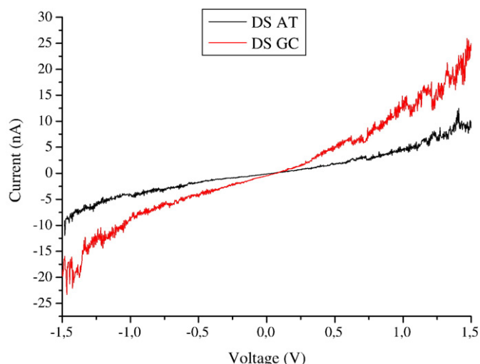
Fig. 3. The typical I(V) curves of DNA GC 32-base double strand (DS GC, see Table 1, ds 1) and DNA AT 32-base double strand (DS AT, see Table 1, ds 2). Set point 0.1 nA, 0.1 V, measured in one voltage direction.
